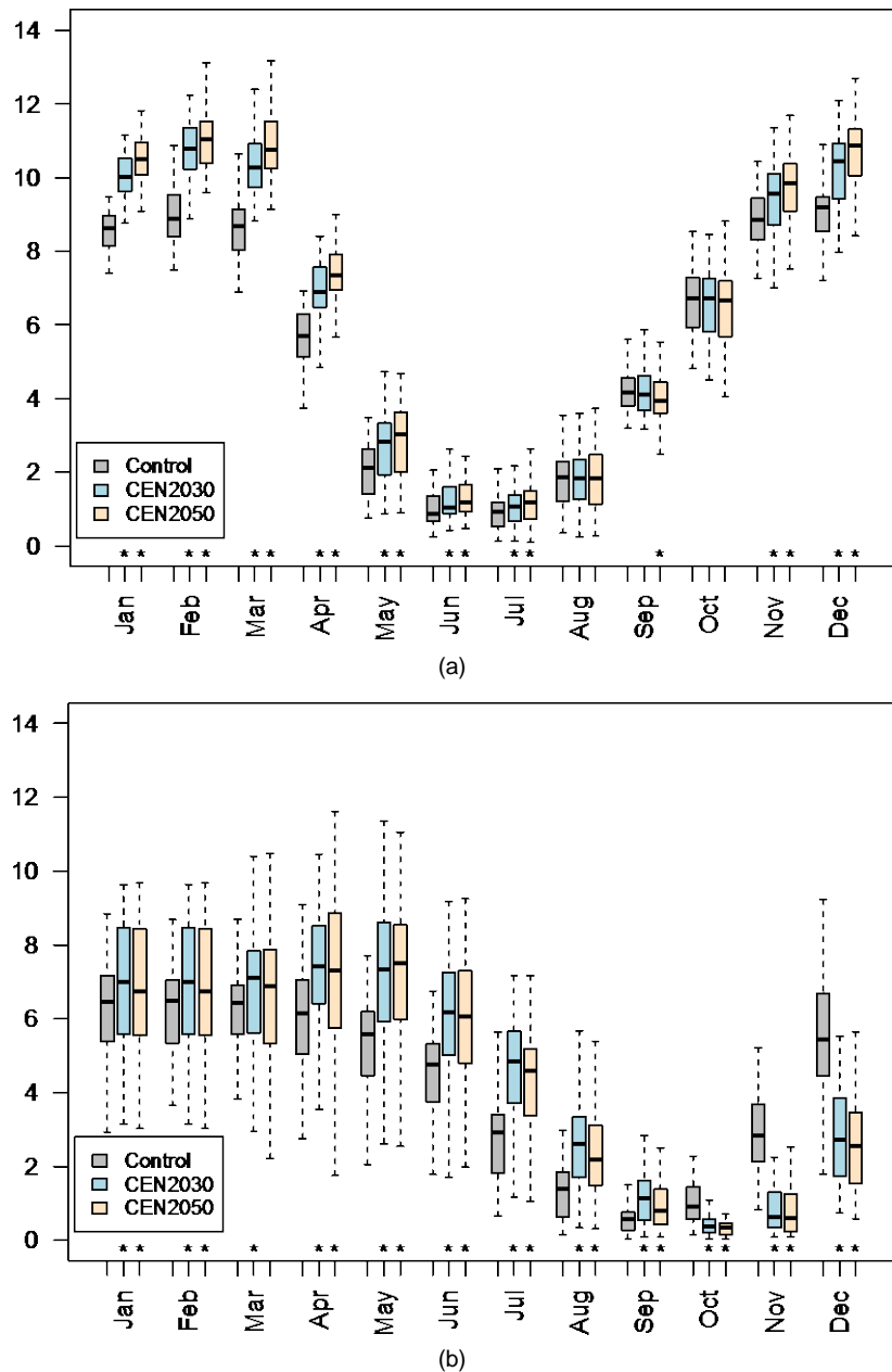
Figure 3. Boxplot of monthly mean precipitation (mm/day) of the control (grey) and deforestation simulations (CEN2030—light blue e CEN2050—beige) at southern-SAMZ (a) and northeast-NEAMZ (b) Amazonia. Asterisks indicate statistically significant differences between control and deforestation simulations ( p < 0.05 , Student's t -test).
