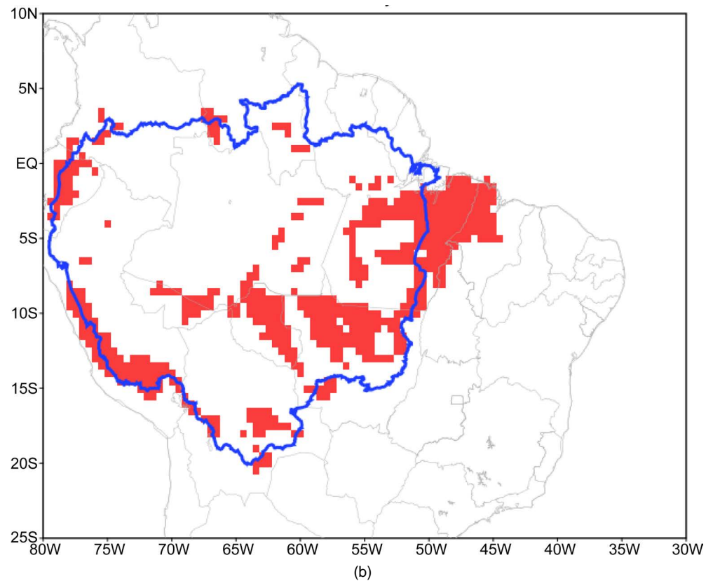
Figure 1. Spatial distribution of the deforested areas used in the perturbed simulations for: (a) 2030 (~28% deforested area) and (b) 2050 (~38% deforested area) according to Aguiar et al. (2015). The red rectangles indicate deforested areas replaced to pasture in the RCM.
